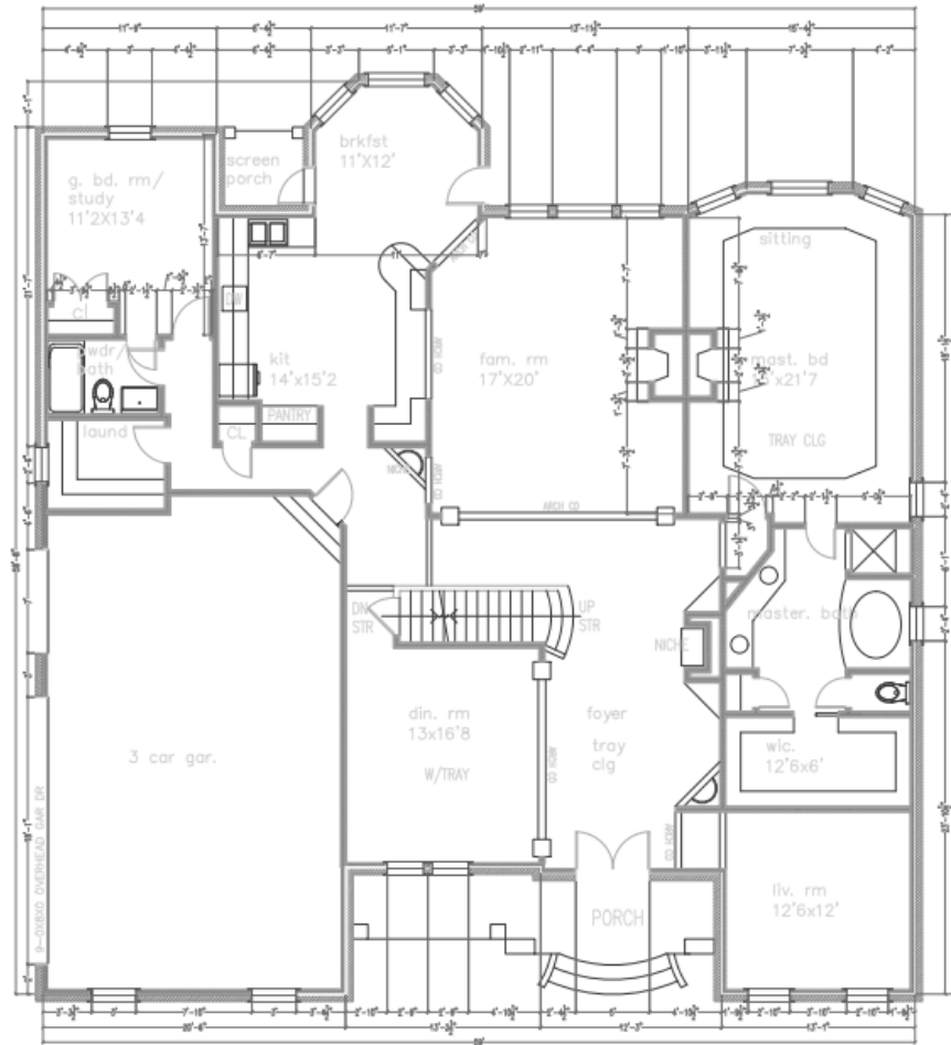
FIRST FLOOR PLAN SCALE : 1/4" = 1'-0" 2372 sq ft
